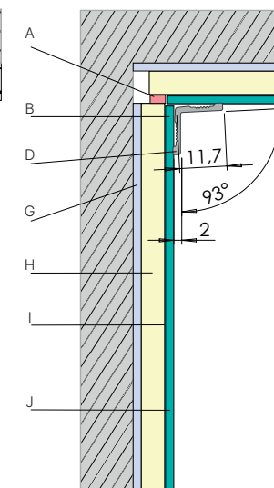
FIN'ANGLE ALU
